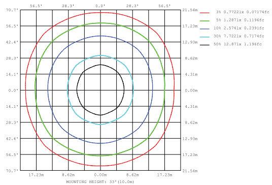
ISOLUX DIAGRAM
